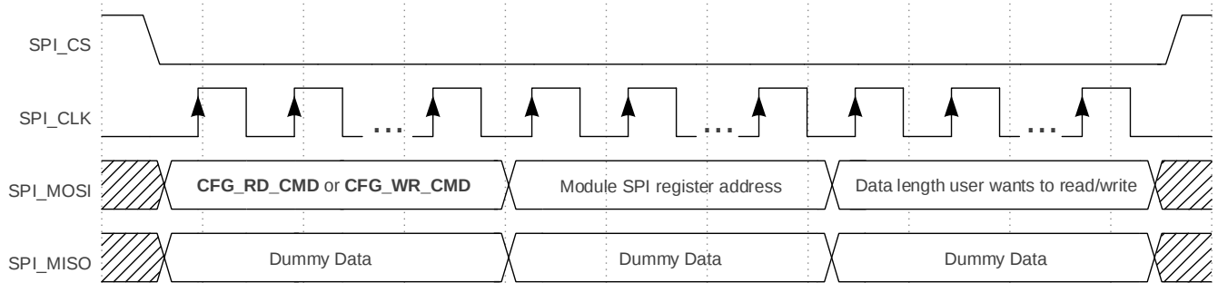
Figure 5: Host Sends CFG_RD_CMD or CFG_WR_CMD
