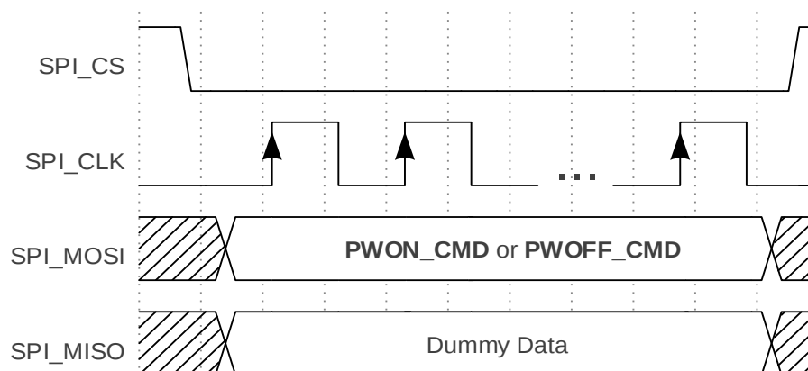
Figure 4: Host Sends PWON_CMD or PWOFF_CMD
