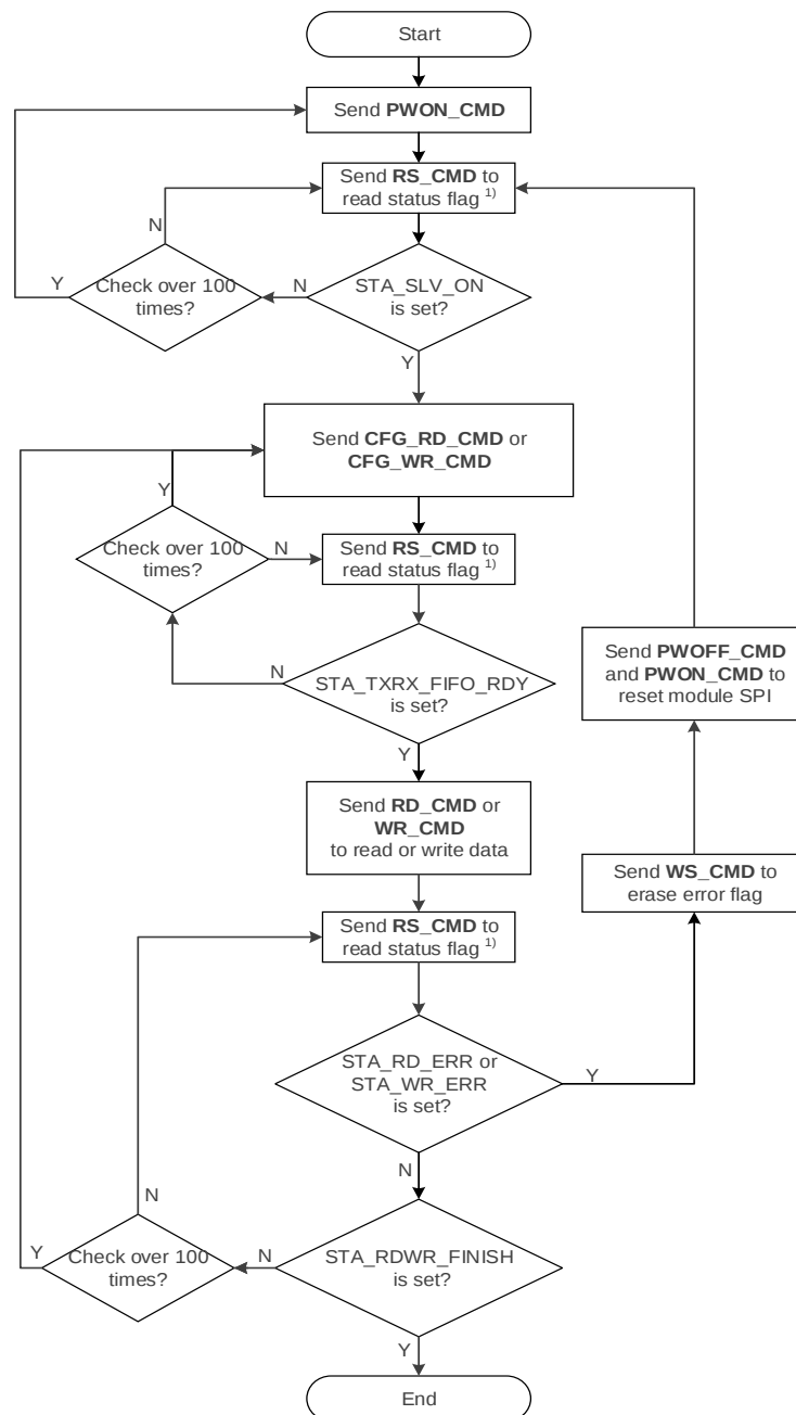
Figure 7: Module SPI Read/Write Flow
