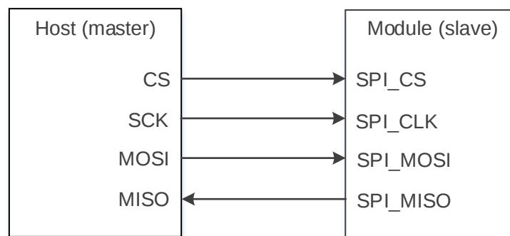
Figure 1: SPI Connection Between Host and Module
