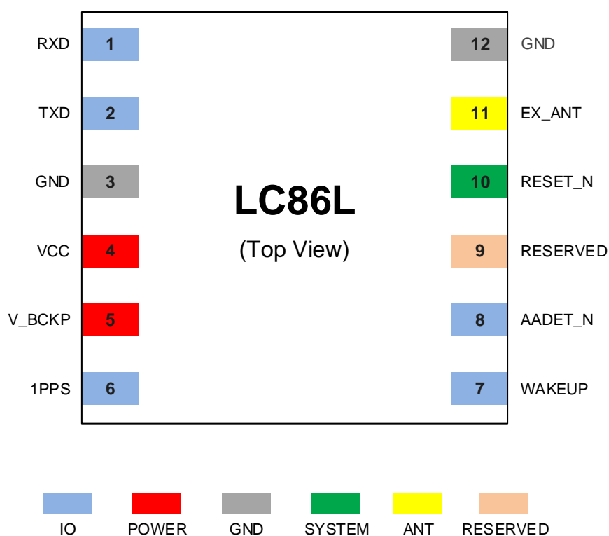
Figure 3: Pin Assignment
